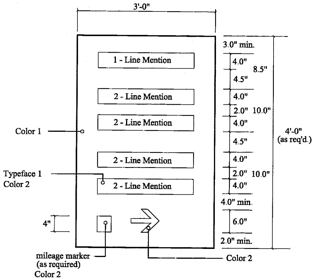
Resource Directional Series/Vertical Scale: 1"=1'-0"
